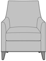
Marino Lounge Chair, with Piping Detail on Base Moasdfadel: MNOLN111 28.5W 28.5D 38H 25AH
