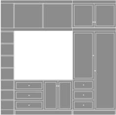
Lancaster Footwall Unit Moasfadel: LAFTWL 111.25W 23.75D 111H
