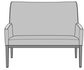
Terrasini Love Seat, Solid Surface Arm Caps, Piping on Base & Back, Concealed Cleanout, Tall Back Model: TER253 47W 29D 40.5H 24.75AH
