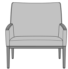
Terrasini Bariatric, with Kwalu Arm Caps, Piping Base & Back, with Concealed Cleanout, Tall Back Model: TERB33 35W 29D 40.5H 25AH
