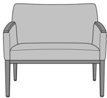
Terrasini Bariatric, with Kwalu Arm Caps, without Piping, with Concealed Cleanout Model: TERB21 35W 26.5D 34H 25AH
