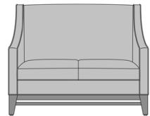
Padova Love Seat, with Piping, Arm 25"H, Double Rail Base Model: PA21B2 54.5W 33.5D 43.5H 25AH
