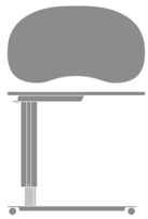
Overbed Table Low Profile Gas Assist U-Base - 32"W x 18"D Jelly Bean Top Model: OTLP4 32W 18D 28.5H
