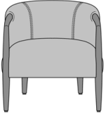
Montedoro Lounge Chair, without Piping on Back & Base Model: MTD10 29W 27D 31H 25AH
